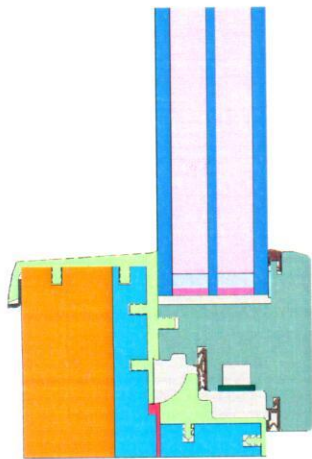
Calculation model
